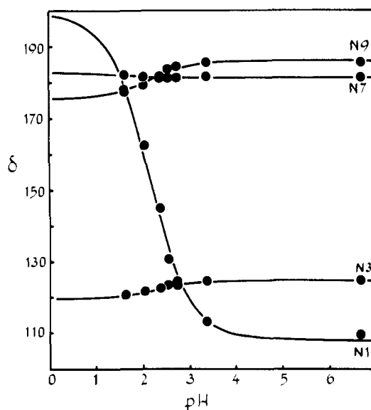
Figure 2. Dependence on the ^{15}\text{N} shifts of purine on pH. The curves for this and succeeding figures were calculated using a nonlinear least-squares fit to the change of shift with pH in which \text{p}K_a and the extremes of chemical shifts at low and high pH were varied to obtain the best fit to the experimental points.
