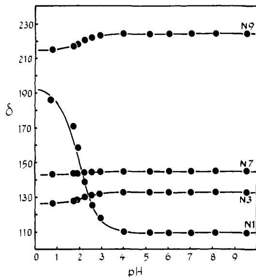
Figure 3. Dependence of the ^{15}\text{N} shifts of 9-methylpurine on pH.
