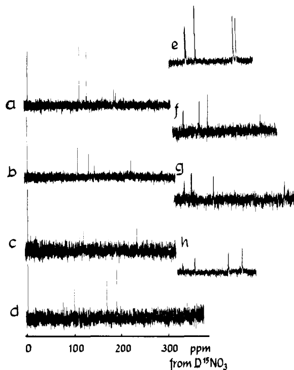
Figure 1. The ^{15}\text{N} NMR proton-decoupled spectra of aqueous solutions of (a) purine, (b) 9-methylpurine, (c) 7-methylpurine, (d) purine in dimethyl sulfoxide, and their proton-coupled spectra e, f, g, and h, respectively.
