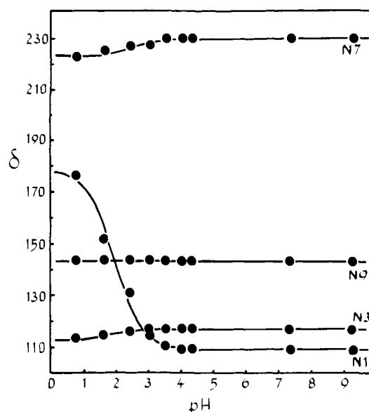
Figure 4. Dependence of the ^{15}\text{N} shifts of 7-methylpurine on pH.
